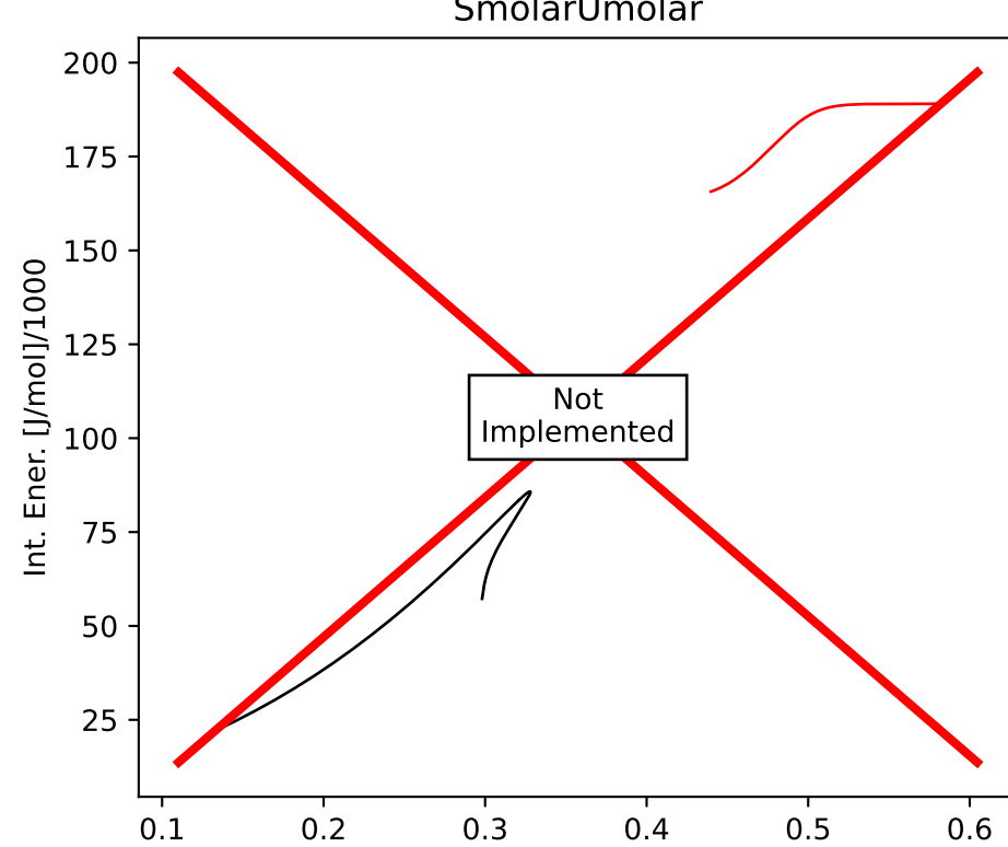
SmolarUmolar
