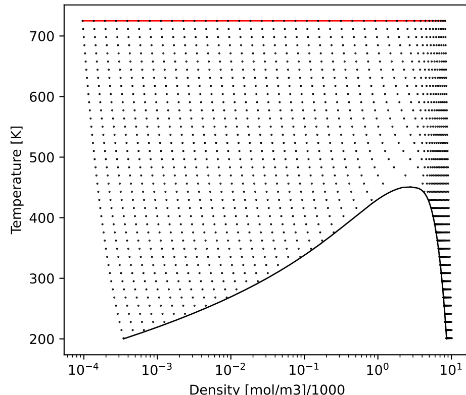
SmolarT
