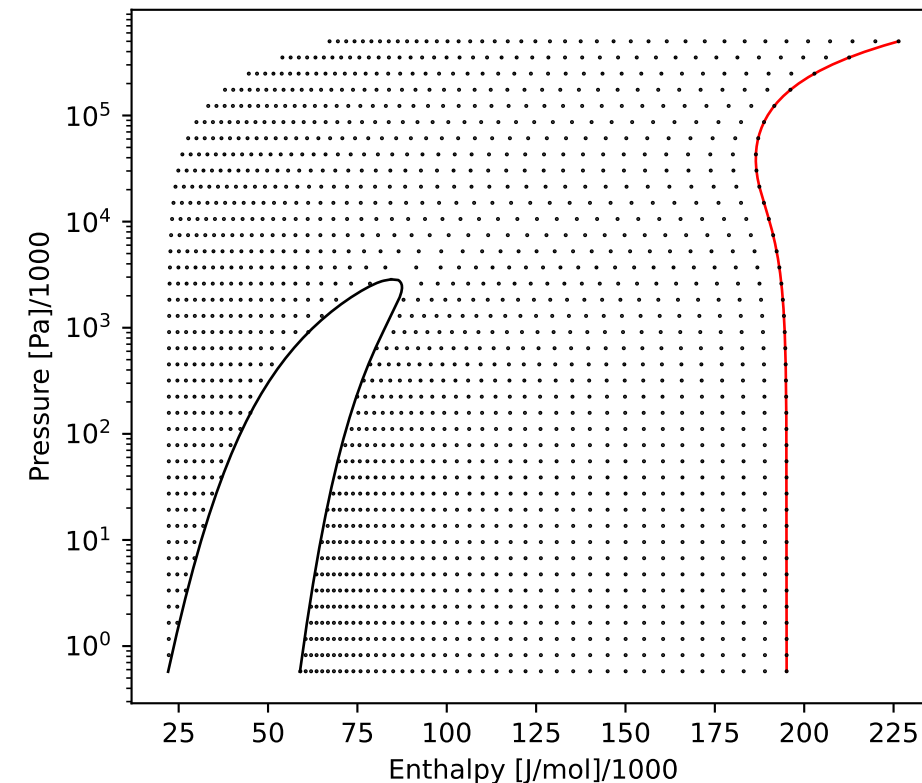
PUmolar
