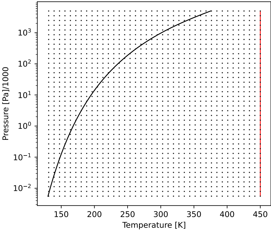
PSmolar
