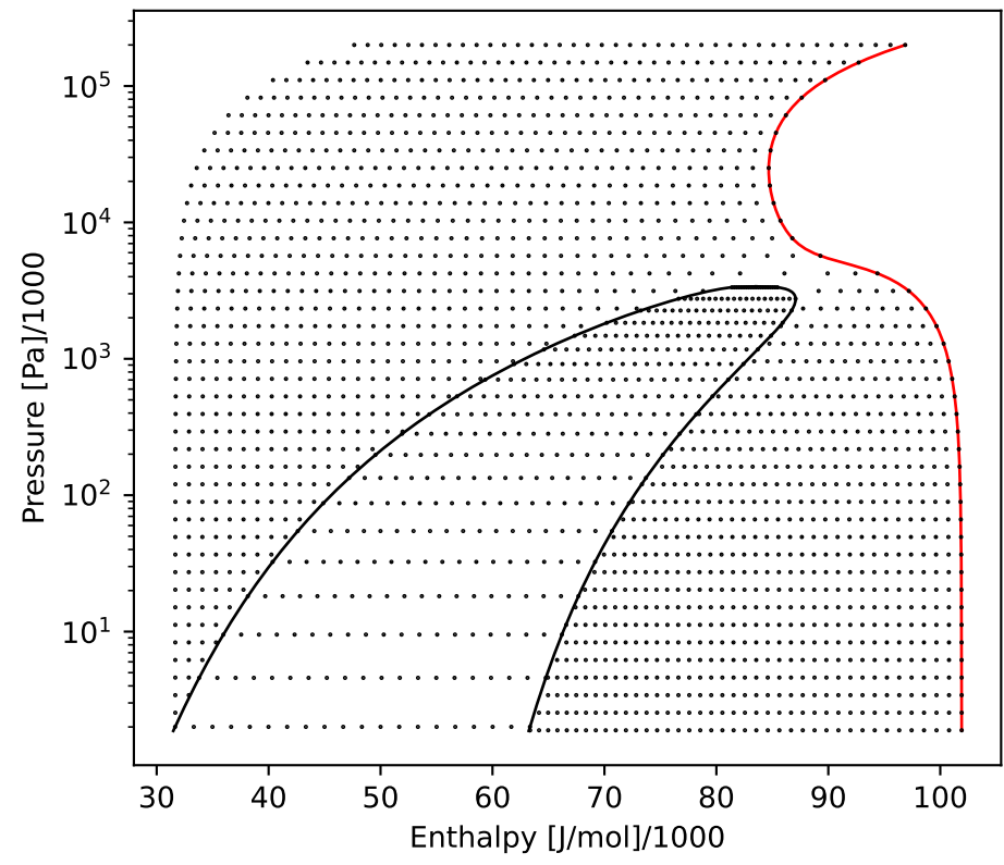
PUmolar
