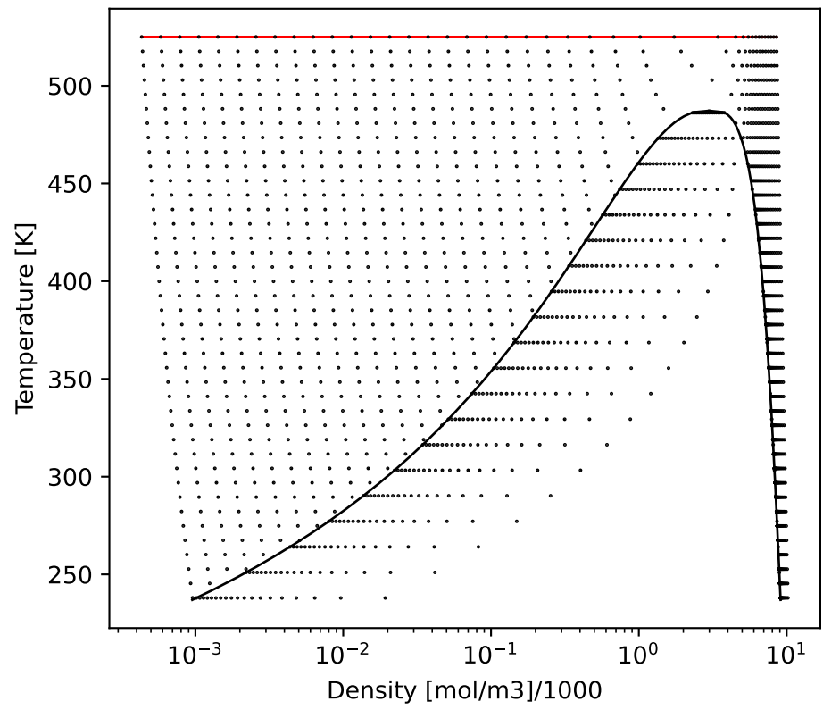
SmolarT
