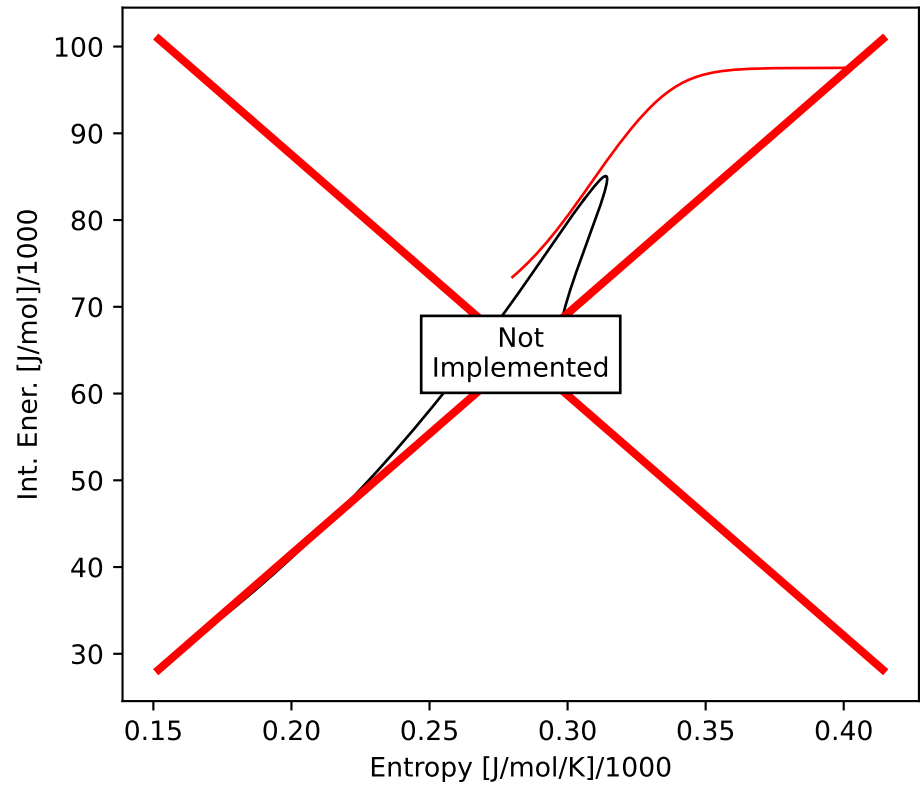
SmolarUmolar
