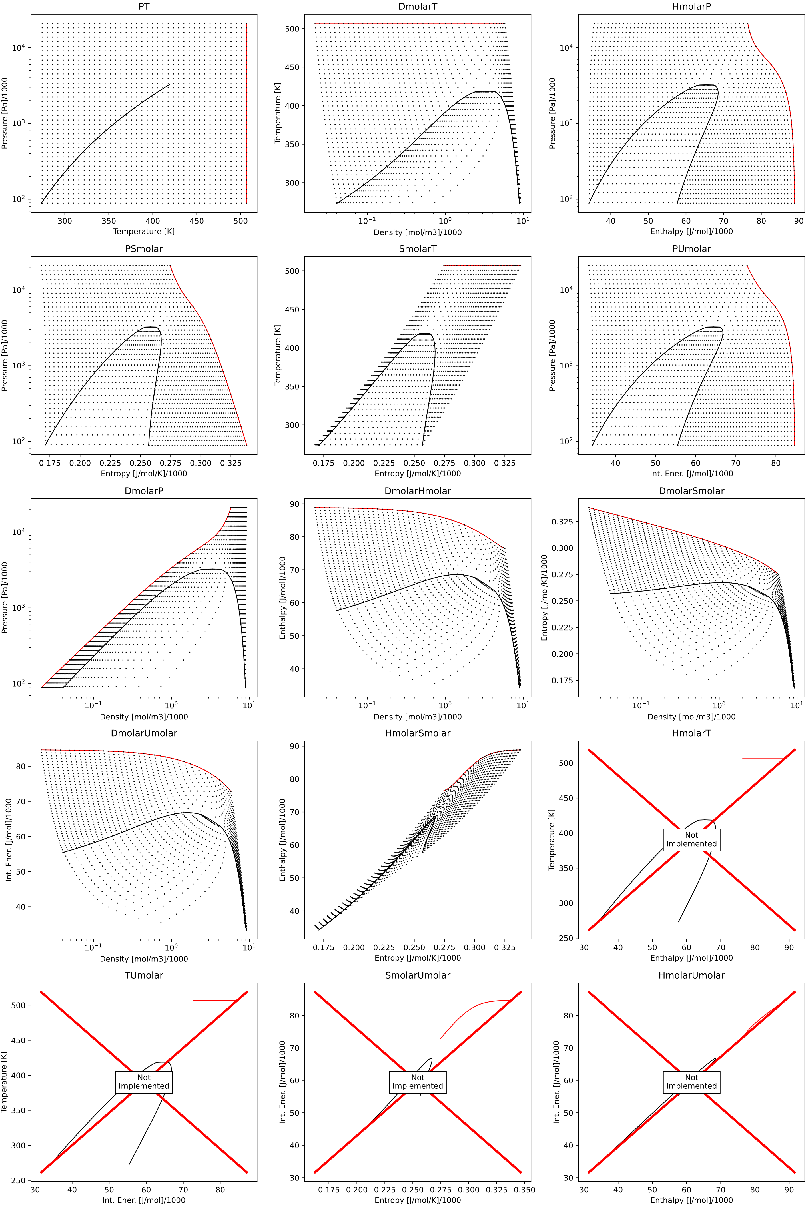
Consistency plots for R114
