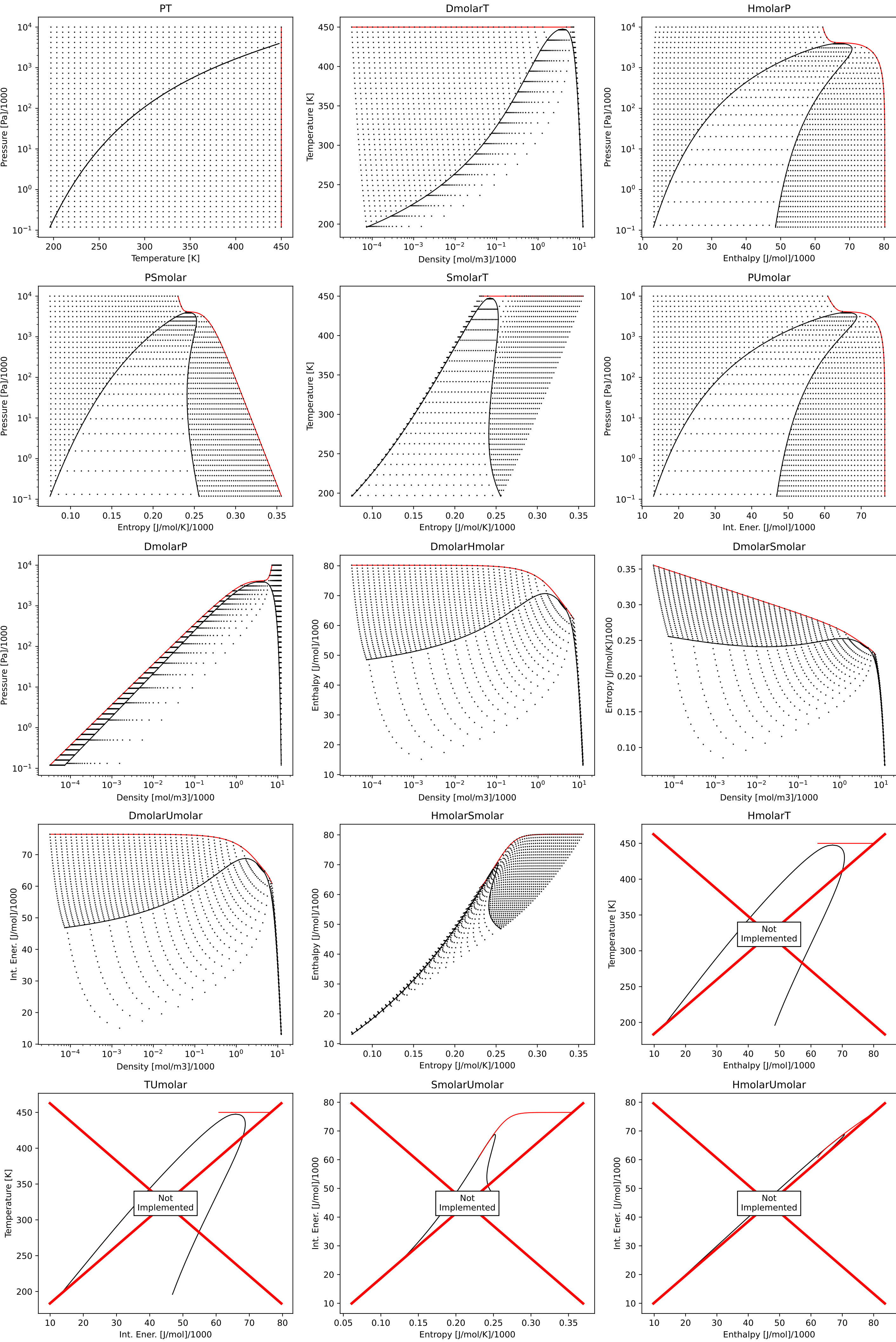
Consistency plots for R245ca
